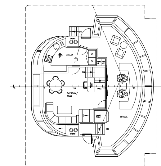
BRIDGE DECK
