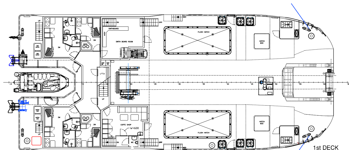
1st DECK
