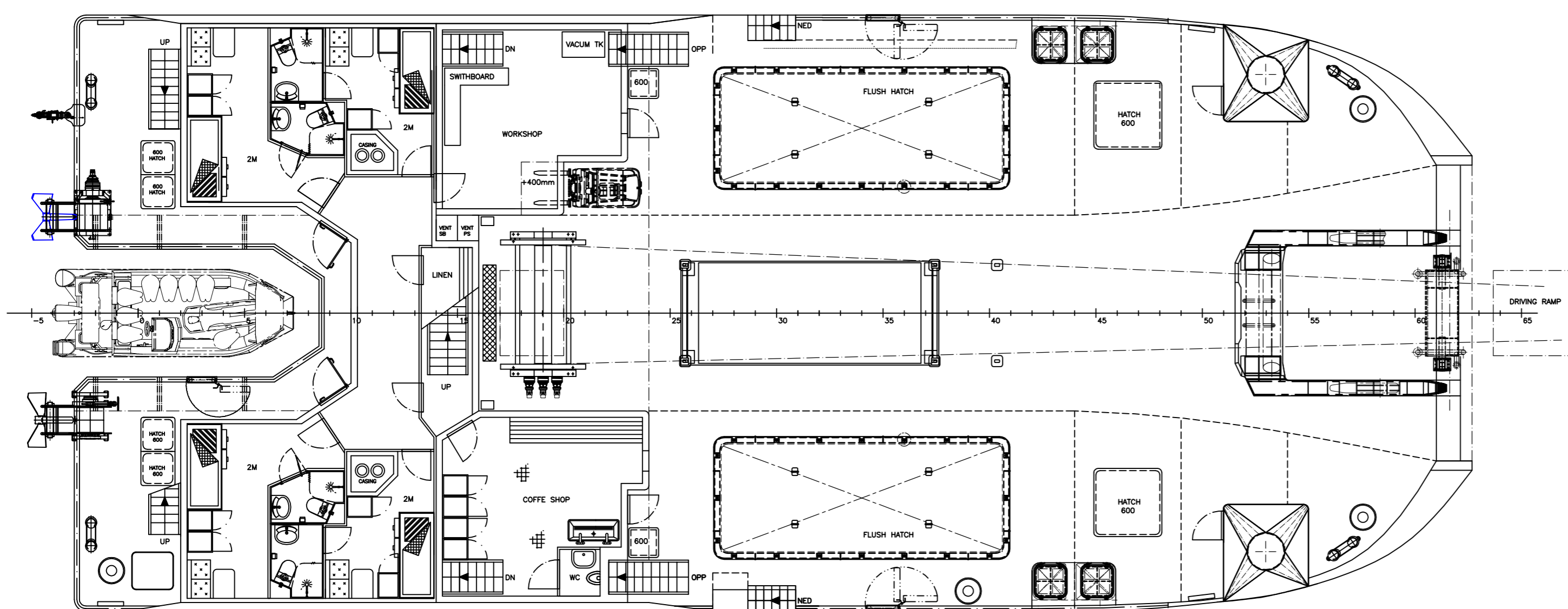
1st DECK
