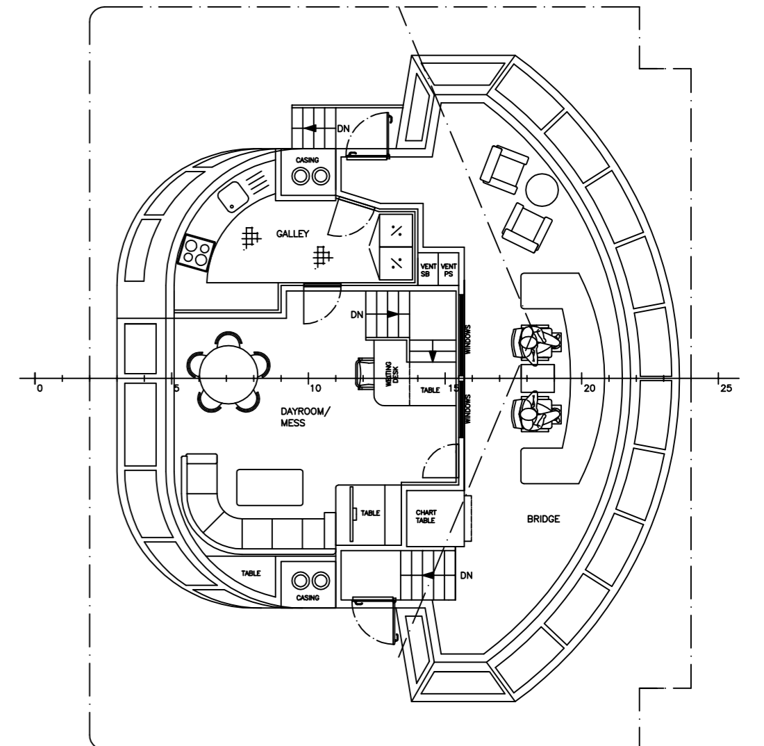
BRIDGE DECK
